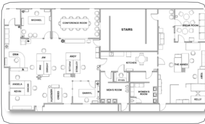
Electrical Layout Design
