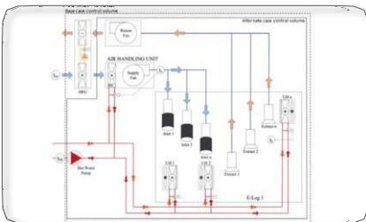
HVAC Design
