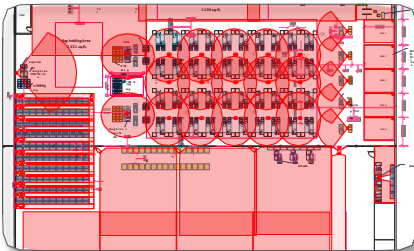
CCTV Design
